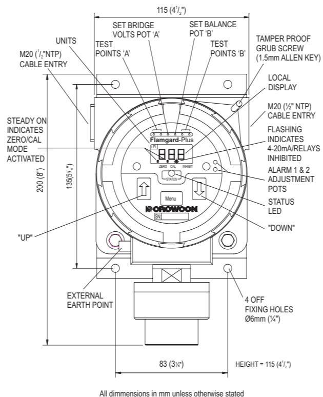
Diagram 1: Flamgard Plus general arrangement
