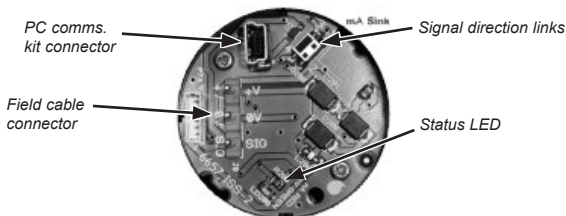
Diagram 5: Signal direction jumper location.
