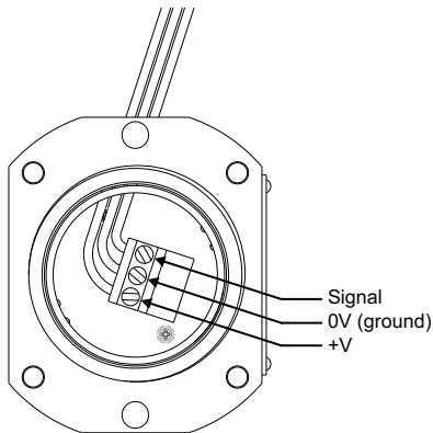
Diagram 4: IREX rear view with back-plate removed
