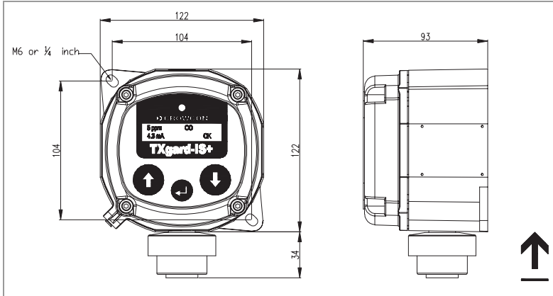
Figure 2.1: TXgard-IS+ dimensions
