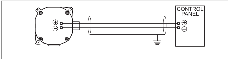
Figure 2.3: Electrical connections for safe area
