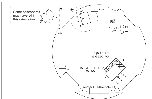
Figure 2.2: Baseboard
